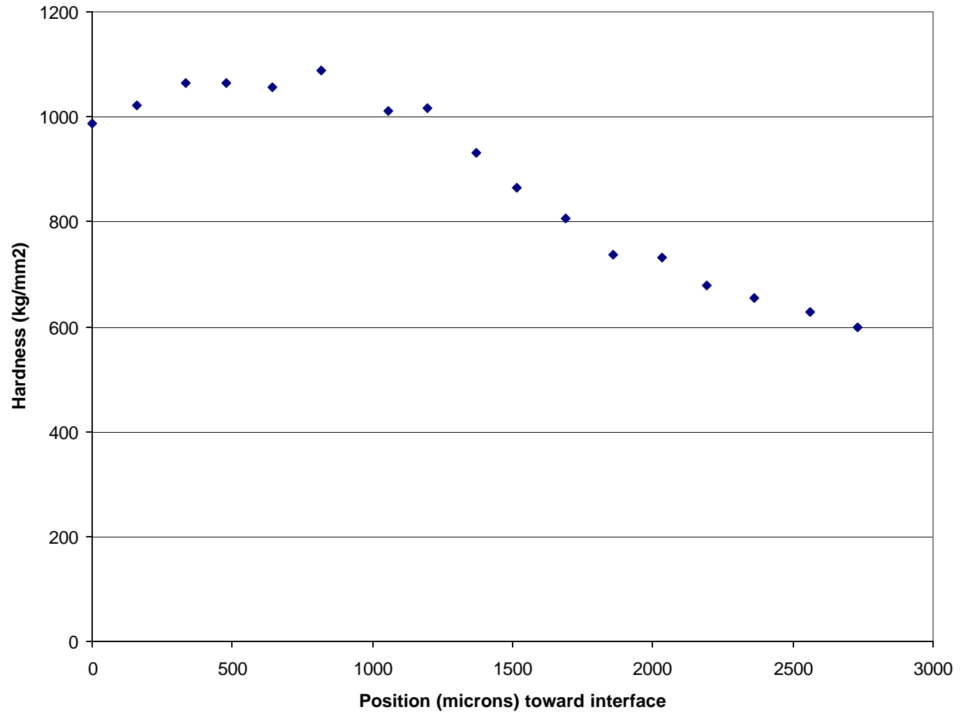
Hardness variation toward Interface (Cut 1)
