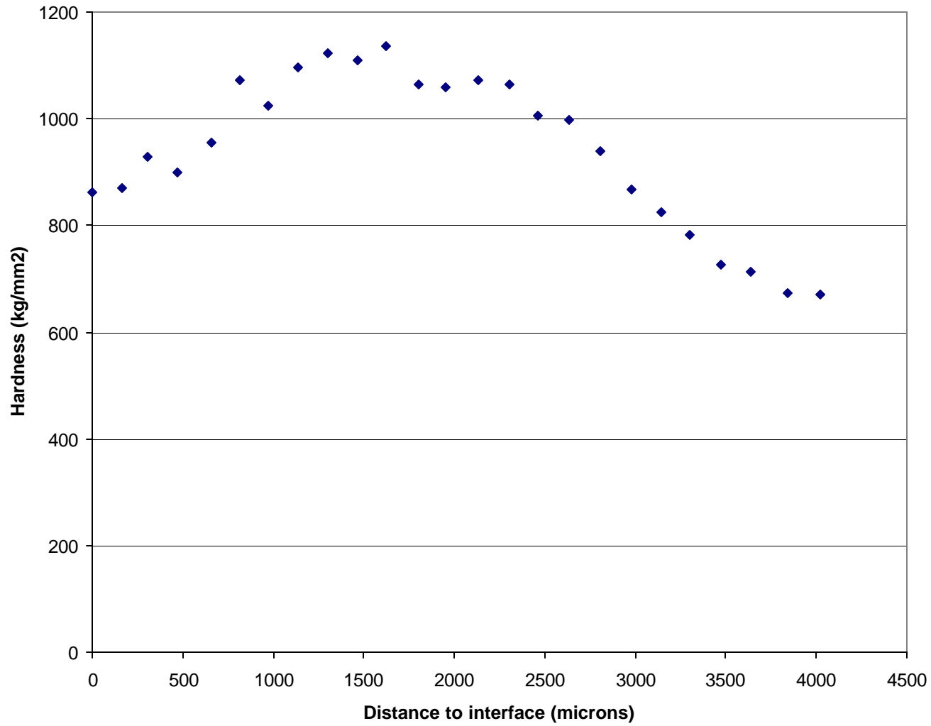
Hardness variation toward interface (Cut 3)
