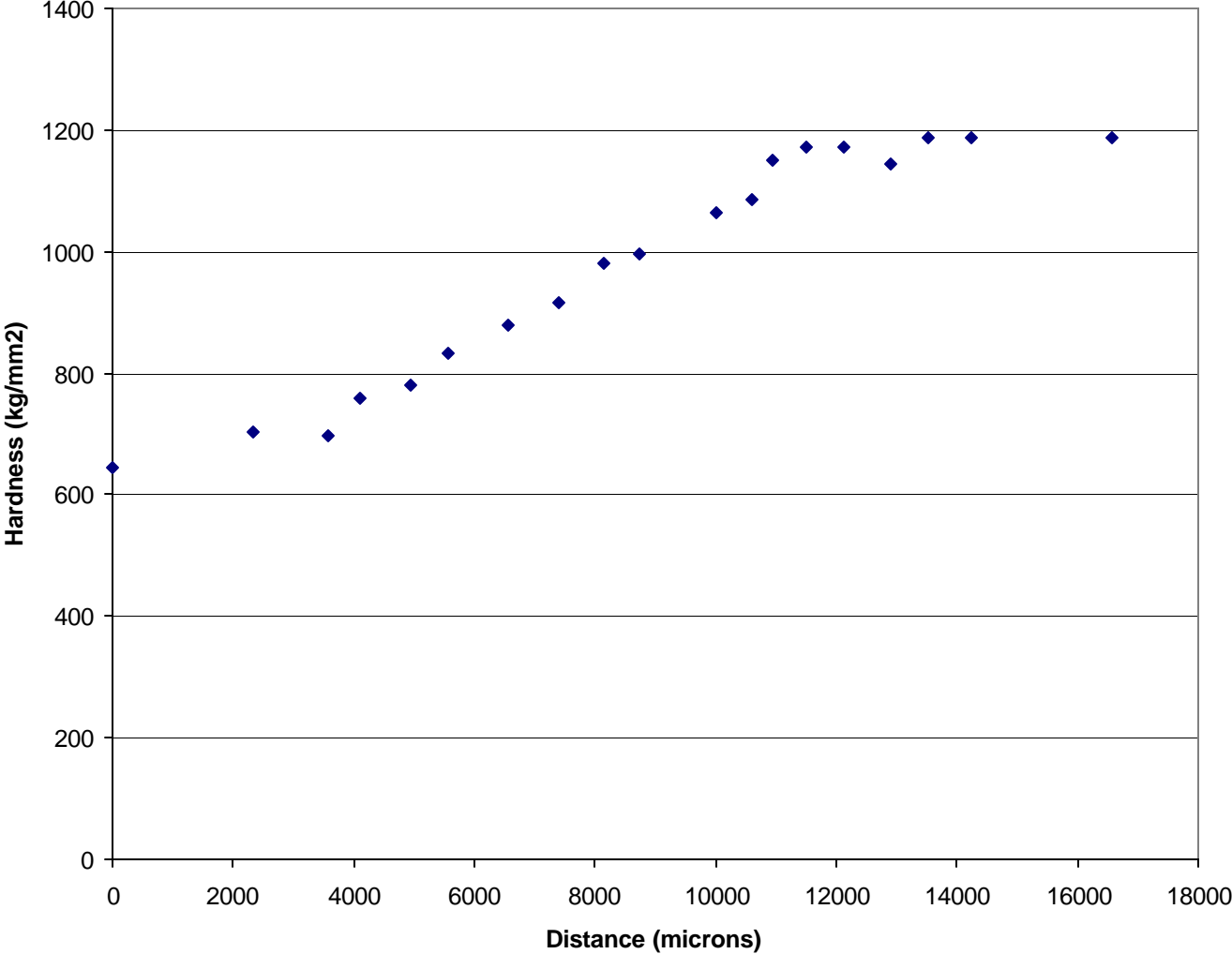
Hardness for SLAC target (Cut 1)
