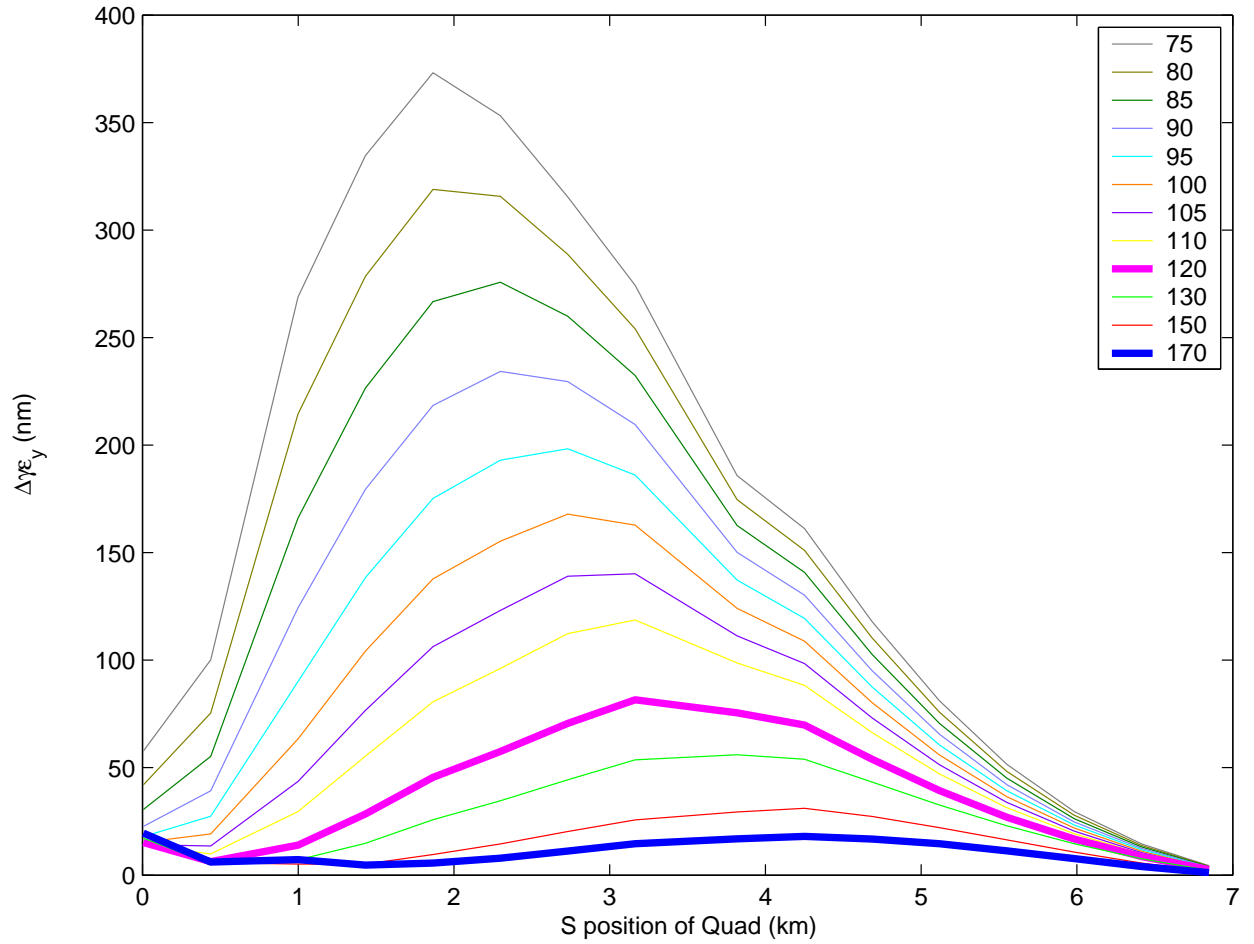
Figure 9: End-linac emittance growth for 1 \mu\text{m} offsets of various quads in the linac, various final energy switch points, plotted as a function of the quadrupole s position. Nominal and new optimal cases are indicated by thicker lines.
