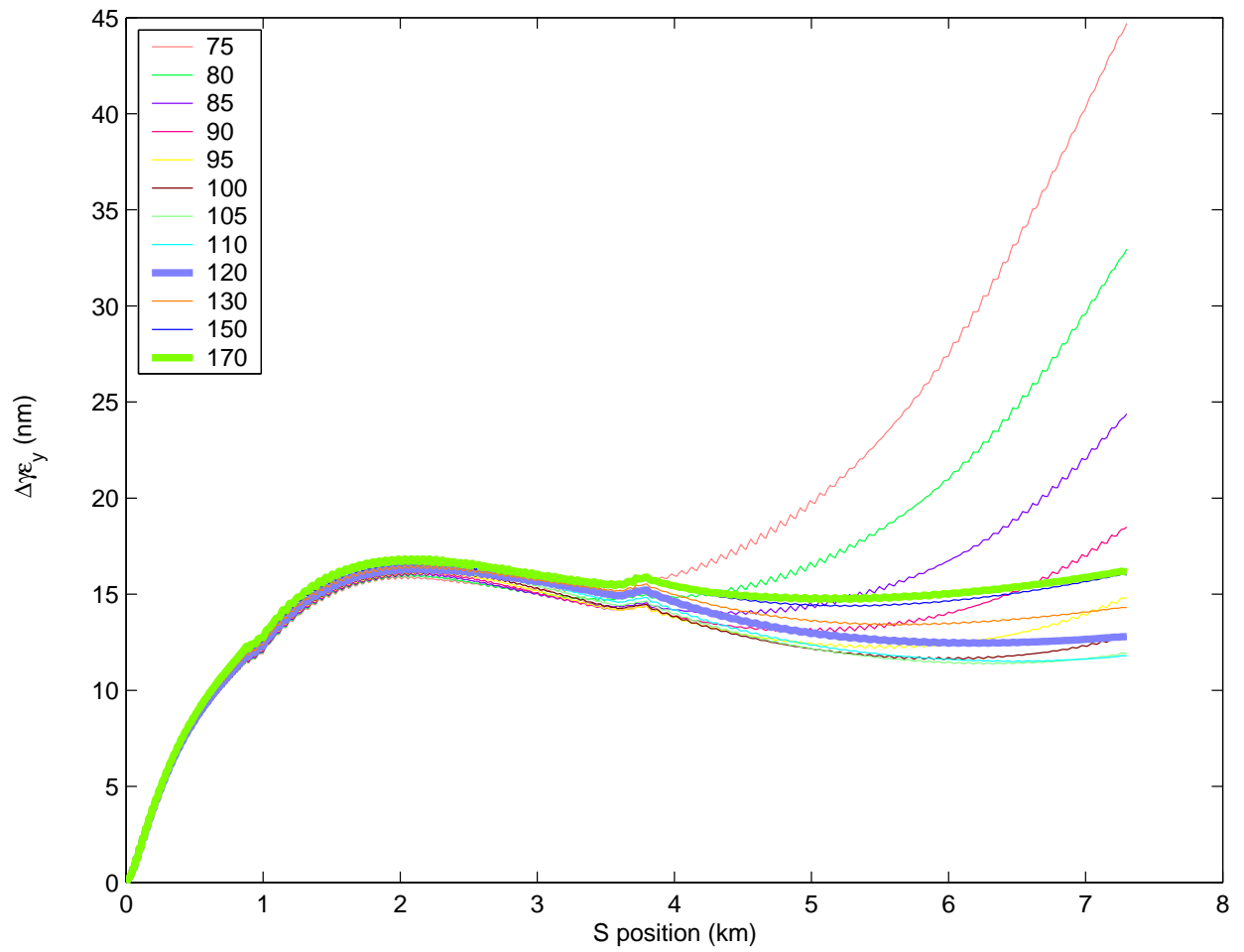
Figure 8: Emittance growth versus s for a 1 \sigma_y initial offset, various final switch energies. Nominal and new optimal cases are indicated by thicker lines.
