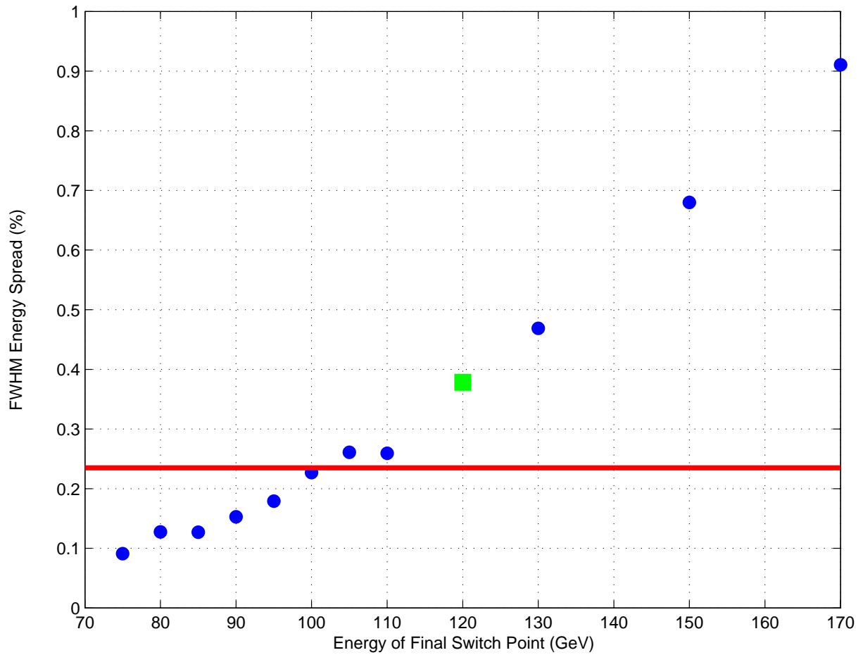
Figure 6: Full width at half maximum energy spread, NLC beam at the end of the linac for various final energy switches. The FWHM of the TESLA beam is also shown for comparison (red line).
