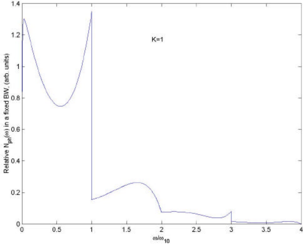
Figure 2: The universal photon number spectrum, h\text{sum}/(w\omega_{10})
