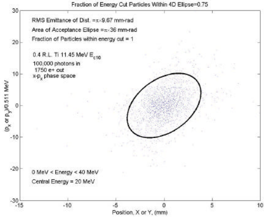
Figure 4: x-p_x phase space distribution of positrons exiting an 0.4 r.l. thick Ti-alloy conversion target. The incident photon spectrum is that of a K=1 undulator with E_{c10} = 11.45 \text{ MeV} and s_x = s_y = 1.09 \text{ mm} .
