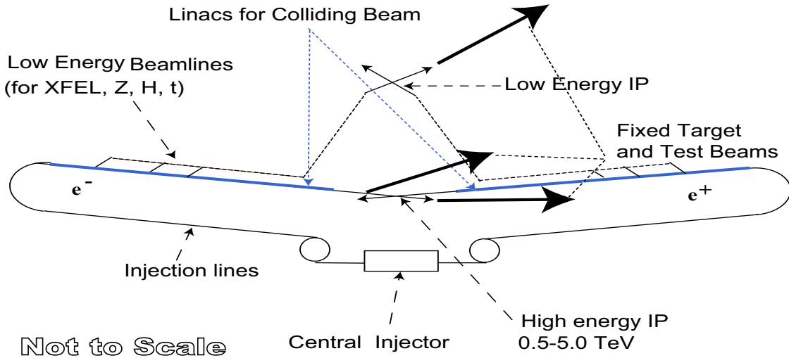
FIGURE 1. Schematic layout for NLC. Note the linac break-out sections at the 50 GeV point (for an XFEL at 0.1\text{\AA} and/or measurements of the Z), and other energies to measure the Higgs and top. Test beam or fixed target facilities could be attached behind either of the IR's or at the end of the electron linac.
