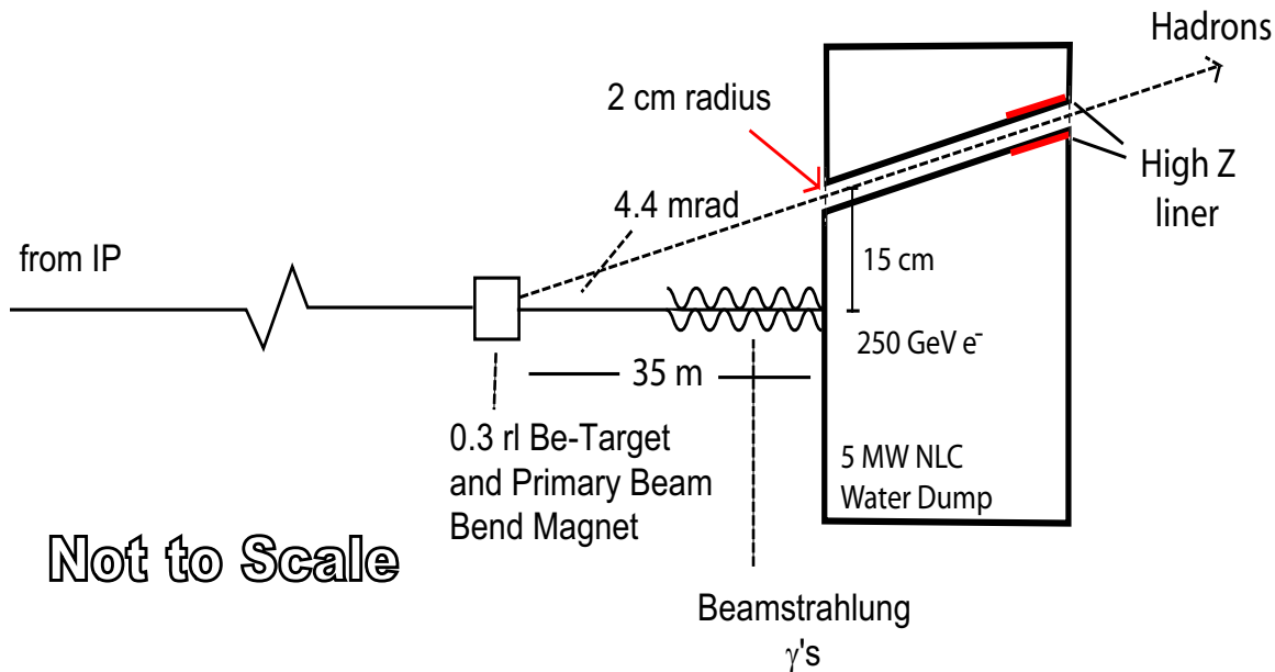
FIGURE 2. Schematic layout of the NLC low energy IR extraction line, including the 5 MW water beam dump and the proposed test beam and fixed target take-off.
