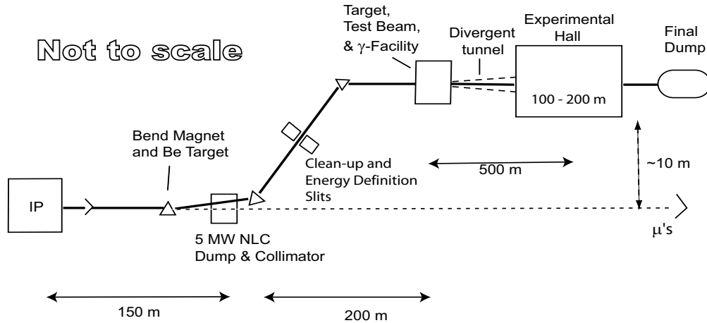
FIGURE 4. Conceptual layout of the fixed target area. The target room doubles as a measurement station for the test beam. The large energies require small scattering angles and, therefore, large drift sections. The target and spectrometer locations are separated by a divergent tunnel to minimize the excavation costs.
