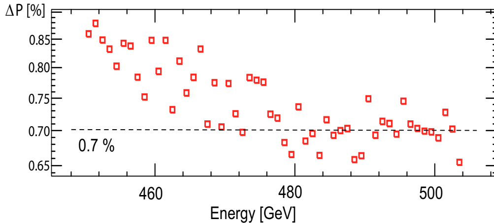
FIGURE 6. Depolarization as a function of disrupted beam energy. The data are for 1 TeV cms.
