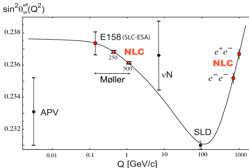
FIGURE 7. The prediction of \sin^2\Theta_W due to radiative corrections, Ref. [18]. The data points labeled APV, \nu N , and SLD are experimental points, the others (red) are predictions and, therefore, are lying on the curve. The NLC colliding beam points and errors are from Ref. [19] and the NLC Møller points and errors are from Ref. [20].
