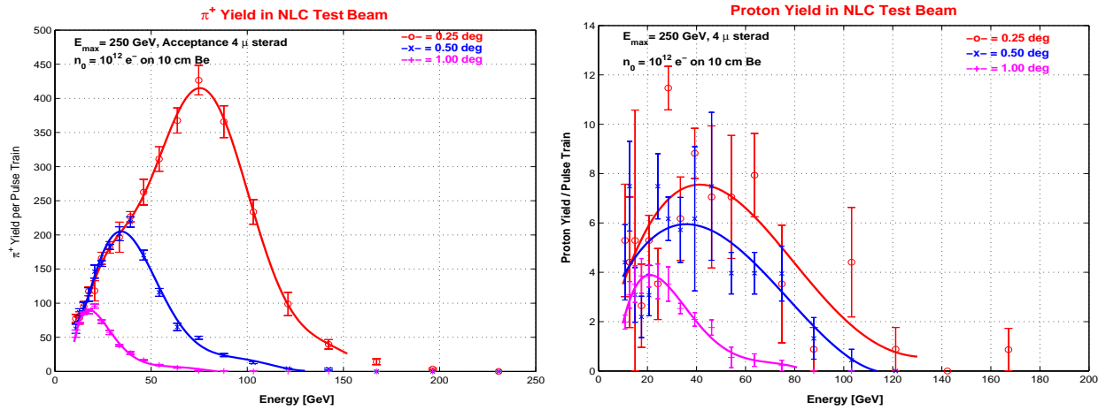
FIGURE 3. Pion and proton yields into 4 \mu\text{sr} solid angle and \Delta P/P = 4\% per nominal NLC pulse train, for three angles, calculated with FLUKA [10]. The yield at low energies is sufficient at all angles shown; simulations with more test particles will be performed in the future to explore the high energy region at larger angles with greater precision.
