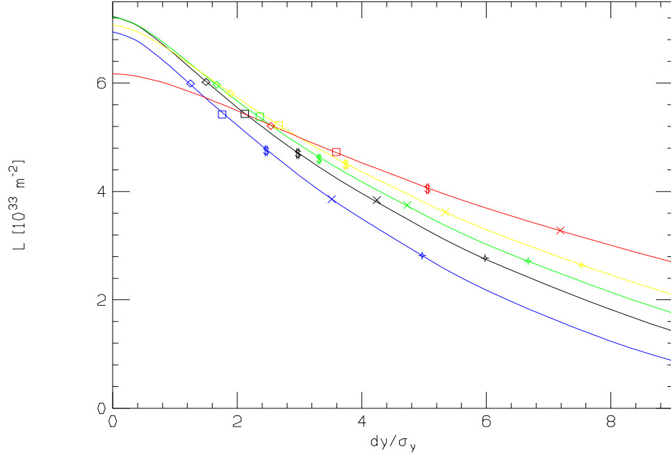
FIGURE 3. Luminosity (per bunch) for y -scans, shown versus dy/\sigma_y , for several vertical beam sizes, with horizontal beam size reduced to \sigma_x = 270 nm. Curves are shown for \sigma_y = 2.88 nm (red), \sigma_y = 3.88 nm (yellow), \sigma_y = 4.38 nm (green), \sigma_y = 4.88 nm (black), \sigma_y = 5.88 nm (blue). The diamonds are the points (one on each curve) for which the beam-to-beam offset is about \frac{\sigma_{y0}}{2} = 7.3 nm. The squares are the points for which the beam-to-beam offset is about \sqrt{2} \cdot \frac{\sigma_{y0}}{2} = 10.3 nm. The $'s are the points for which the beam-to-beam offset is about \sigma_{y0} = 14.6 nm. The X's are the points for which the beam-to-beam offset is about \sqrt{2} \cdot \sigma_{y0} = 20.7 nm. The +'s are the points for which the beam-to-beam offset is about 2 \cdot \sigma_{y0} = 29.2 nm.
