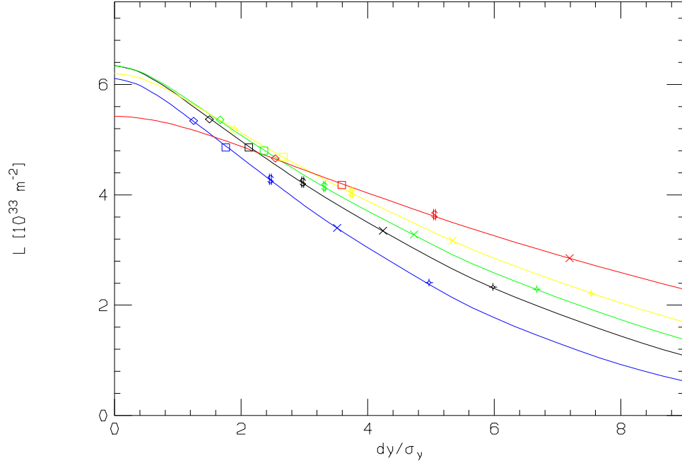
FIGURE 2. Luminosity (per bunch) for y -scans, shown versus dy/\sigma_y , for several vertical beam sizes, with horizontal beam size reduced to \sigma_x = 300 nm. Curves are shown for \sigma_y = 2.88 nm (red), \sigma_y = 3.88 nm (yellow), \sigma_y = 4.38 nm (green), \sigma_y = 4.88 nm (black), \sigma_y = 5.88 nm (blue). The diamonds are the points (one on each curve) for which the beam-to-beam offset is about \frac{\sigma_{y0}}{2} = 7.3 nm. The squares are the points for which the beam-to-beam offset is about \sqrt{2} \cdot \frac{\sigma_{y0}}{2} = 10.3 nm. The $'s are the points for which the beam-to-beam offset is about \sigma_{y0} = 14.6 nm. The X's are the points for which the beam-to-beam offset is about \sqrt{2} \cdot \sigma_{y0} = 20.7 nm. The +'s are the points for which the beam-to-beam offset is about 2 \cdot \sigma_{y0} = 29.2 nm.
