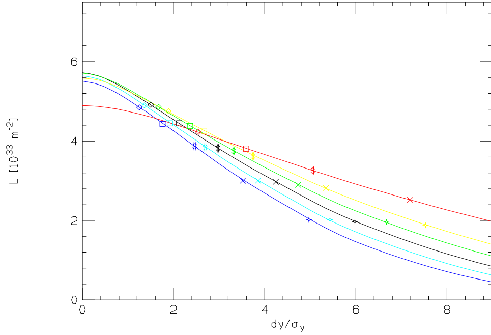
FIGURE 1. Luminosity (per bunch) for y -scans, shown versus dy/\sigma_y , for several vertical beam sizes, with horizontal beam size kept at its nominal value of \sigma_x = 327 nm. Curves are shown for \sigma_y = 2.88 nm (red), \sigma_y = 3.88 nm (yellow), \sigma_y = 4.38 nm (green), \sigma_y = 4.88 nm (black), \sigma_y = 5.38 nm (cyan), \sigma_y = 5.88 nm (blue). The diamonds are the points (one on each curve) for which the beam-to-beam offset is about \frac{\sigma_{y0}}{2} = 7.3 nm. The squares are the points for which the beam-to-beam offset is about \sqrt{2} \cdot \frac{\sigma_{y0}}{2} = 10.3 nm. The $'s are the points for which the beam-to-beam offset is about \sigma_{y0} = 14.6 nm. The X's are the points for which the beam-to-beam offset is about \sqrt{2} \cdot \sigma_{y0} = 20.7 nm. The +'s are the points for which the beam-to-beam offset is about 2 \cdot \sigma_{y0} = 29.2 nm.
