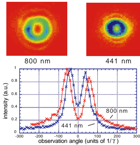
Figure 3: Comparison of two-foil interference at 441 and 800 nm shows expected wavelength dependence.
